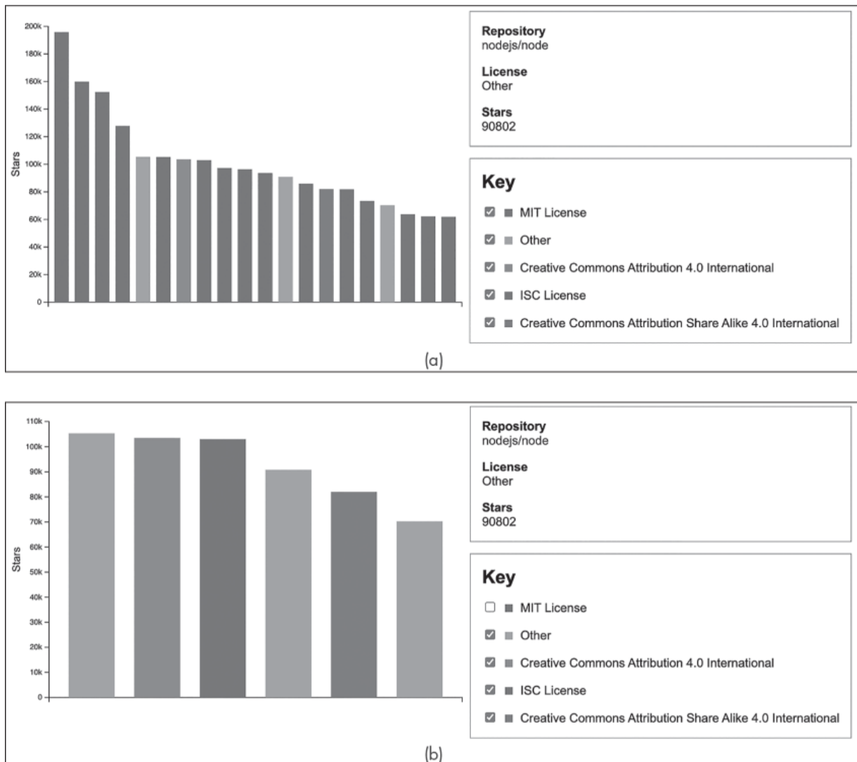
Figure 15-6: The final chart showing all licenses (a) and with the top license hidden (b)
